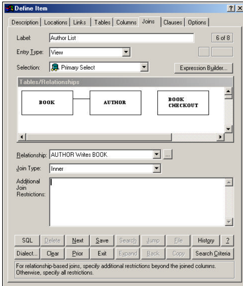
Figure 5-15 Define Dialog Box, View Joins Tab
