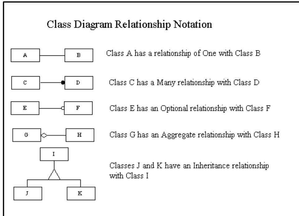
Figure 3-25 Class Relationship Notation
