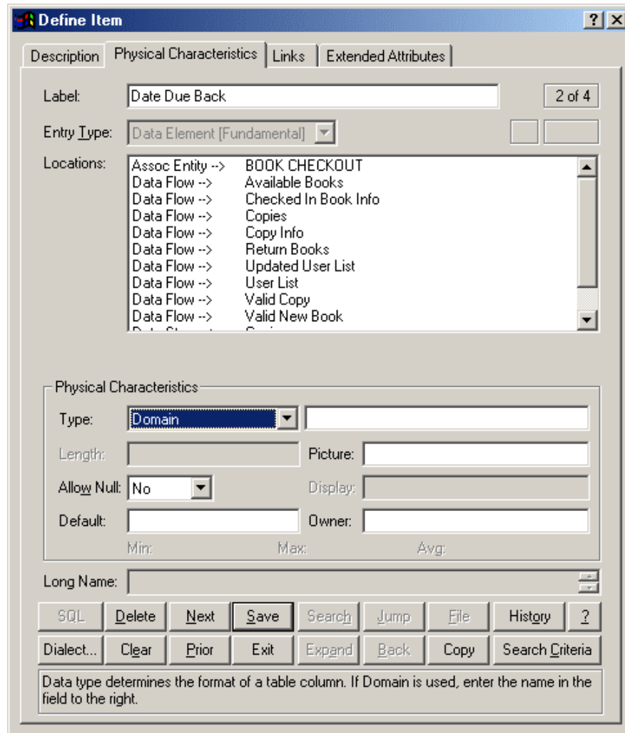
Figure 5-20 Data Element Entry with a Domain
