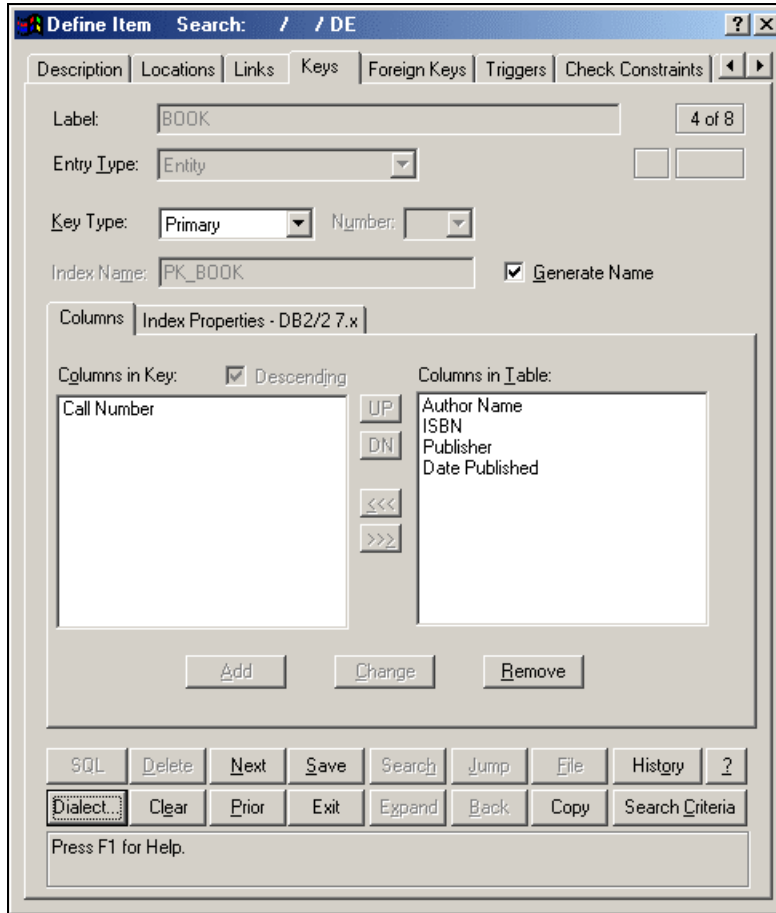
Figure 5-34 Define Dialog Box SQL Schema Generation Information Tabs
