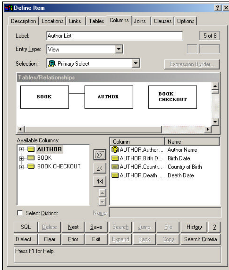
Figure 5-14 Define Dialog Box, View Columns Tab
