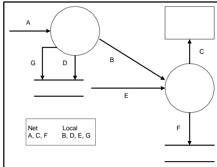
Figure 4-15 Net and Local Data Flows
