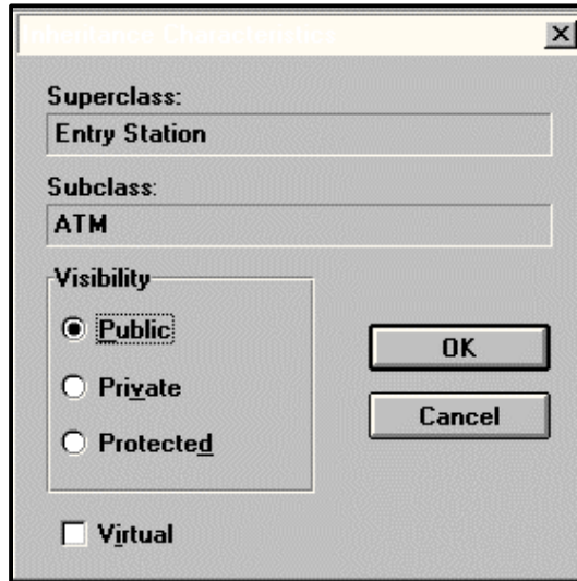
Figure 5-22 Inheritance Characteristics
