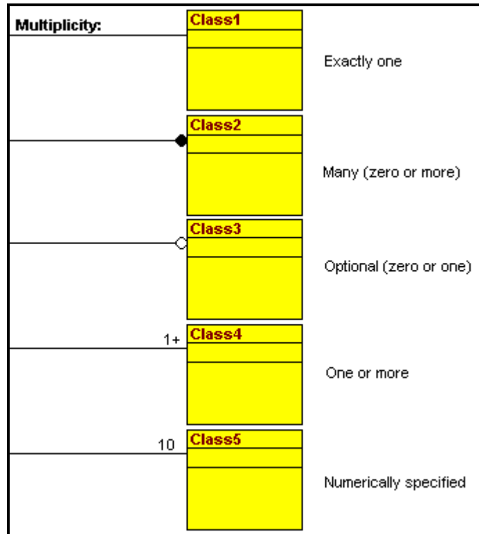
Figure 3-27 UML Relationship Notation
