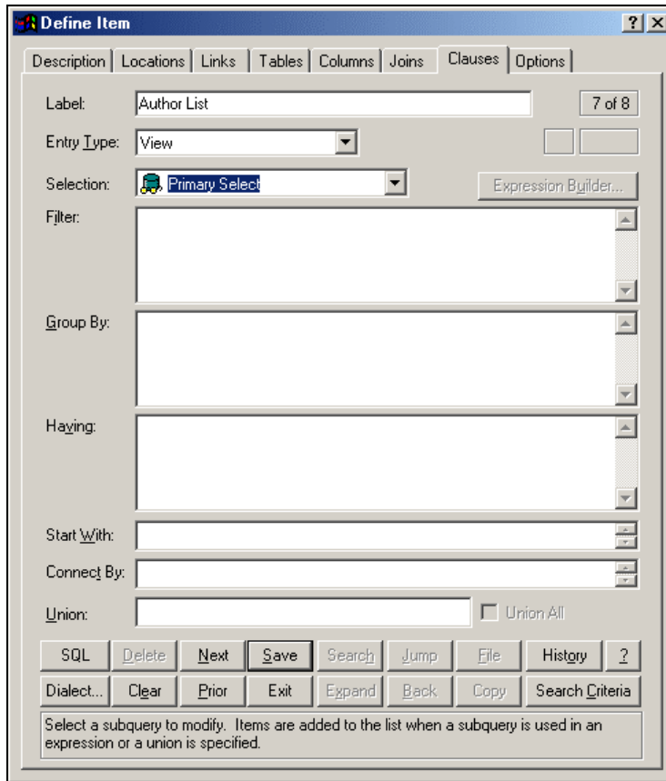
Figure 5-16 Define Dialog Box, View Clauses Tab
