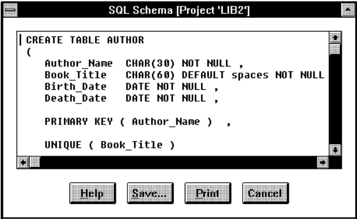
Figure 5-31 Generated SQL Schema
