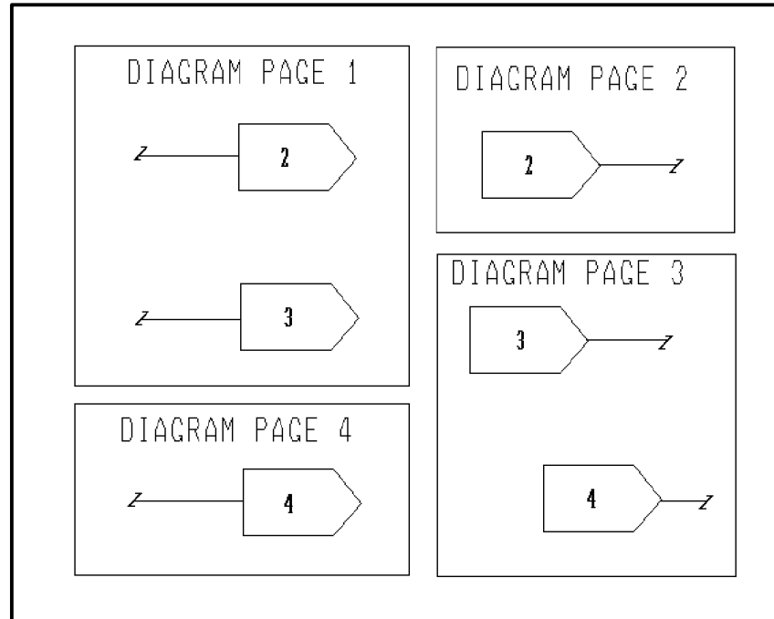
Figure 3-42 Recommended Page Link Symbols for Data Flow
