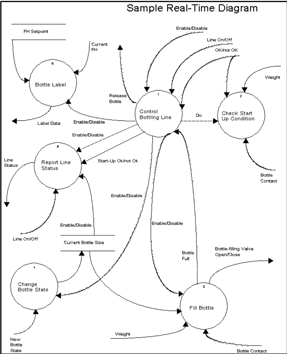
Figure 3-47 Sample Real-Time Diagram
