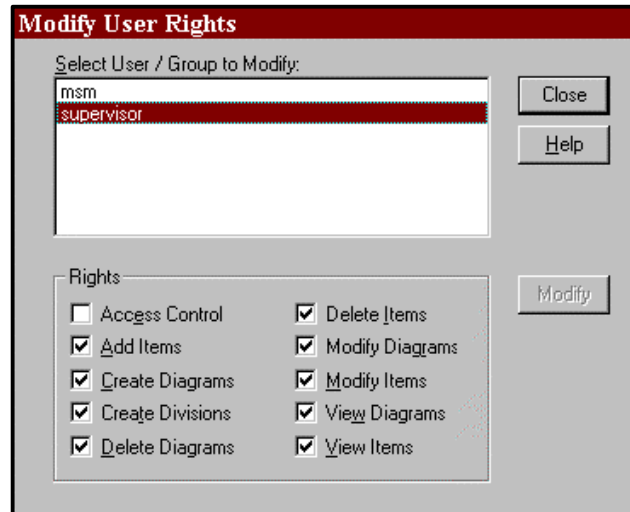
Figure 6-2 Modify User Rights Dialog Box
