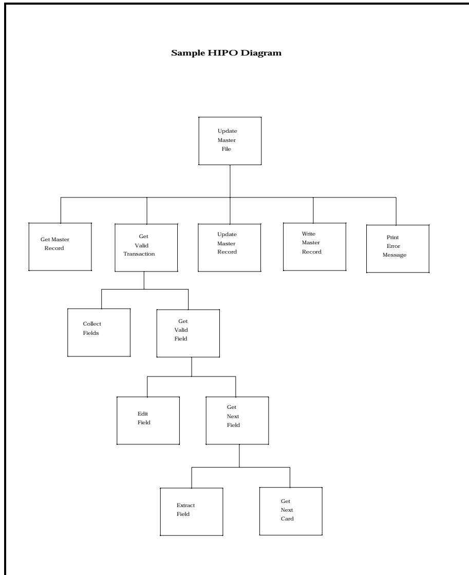
Figure 3-49 Sample HIPO Diagram
