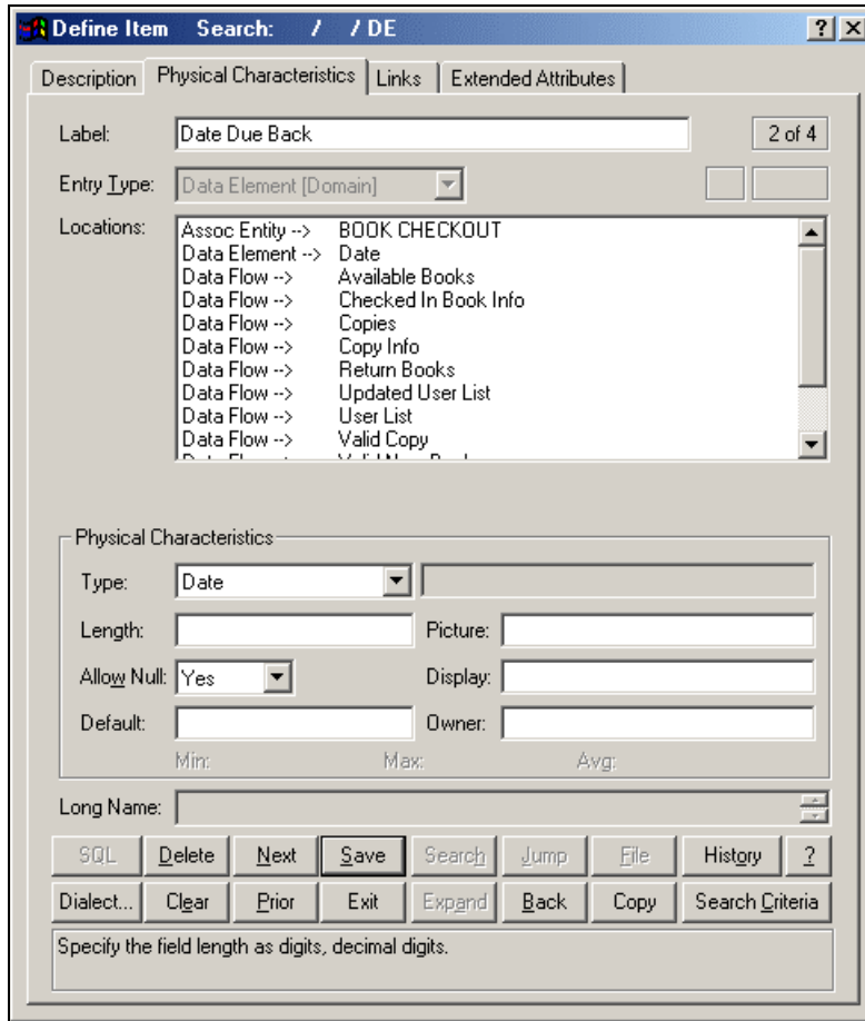
Figure 5-21 Repository Domain Entry
