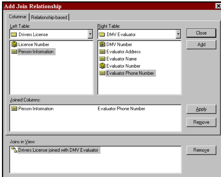
Figure 5-18 Join Relationships Dialog Box, Columnar Tab
