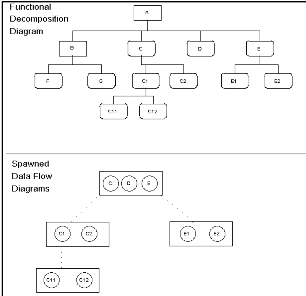
Figure 3-40 DFDs Created by an FDD by Using SPAWN
