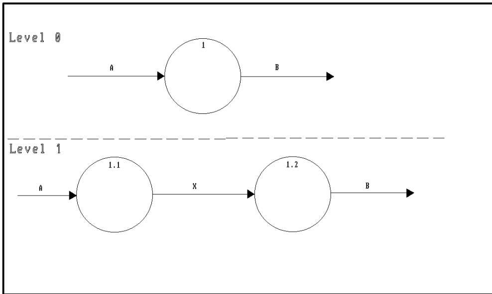
Figure 4-3 Data Flow Balancing
