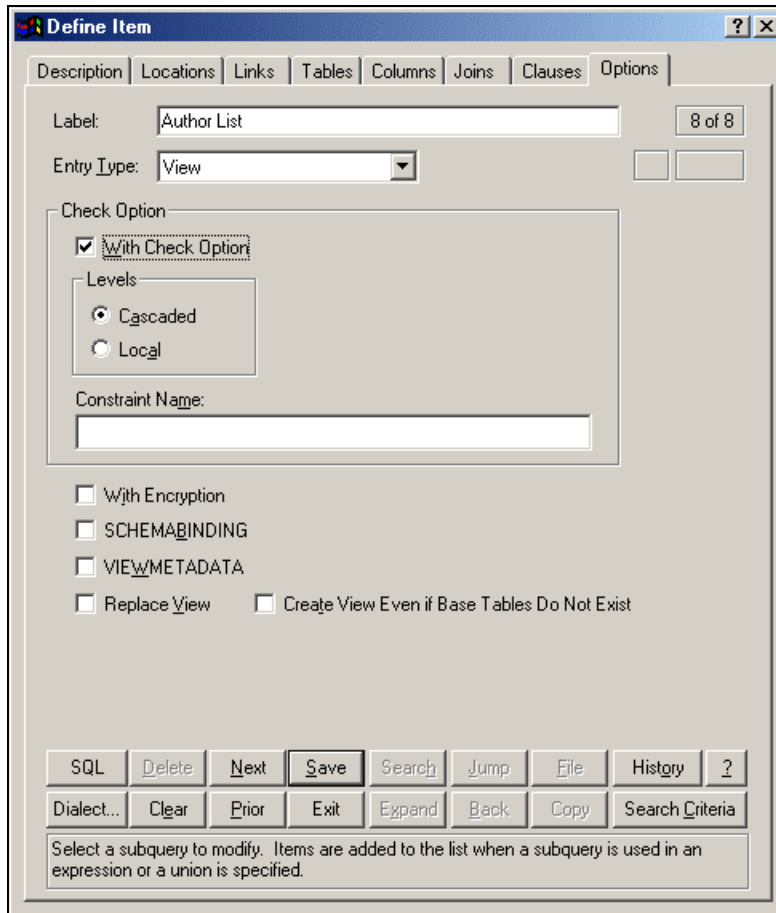
Figure 5-17 Define Dialog Box, View Options Tab
