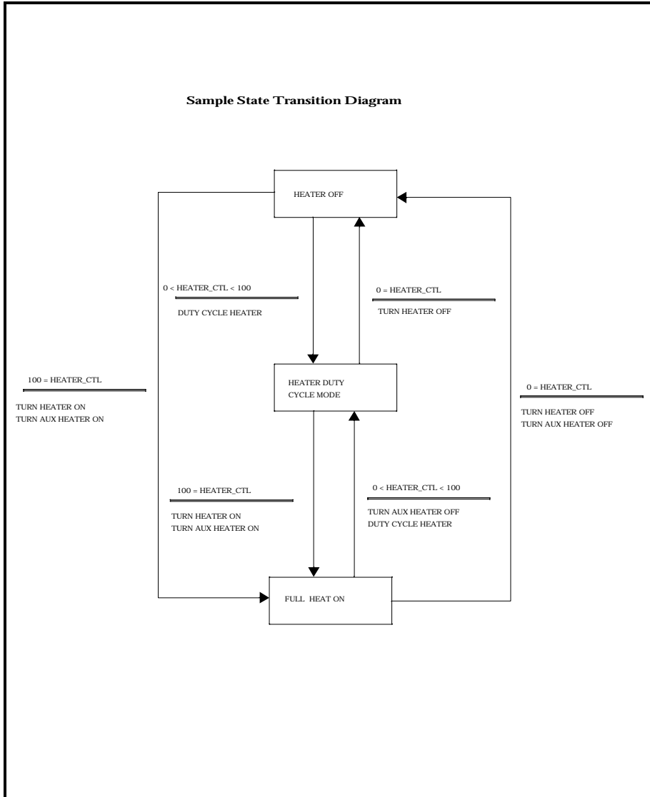
Figure 3-48 Sample State Transition Diagram
