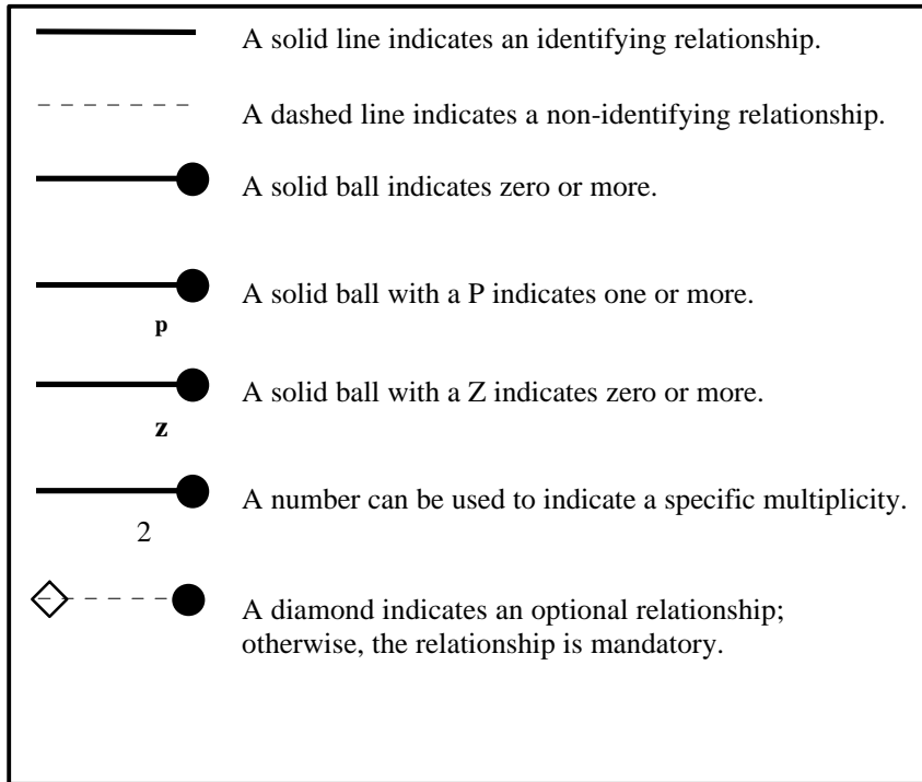
Figure 3-26 IDEF1X Relationship Line Terminators
