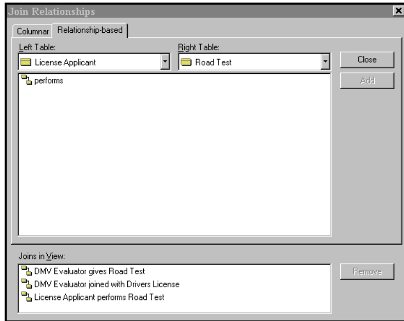
Figure 5-19 Join Relationships Dialog Box, Relationship-based Tab
