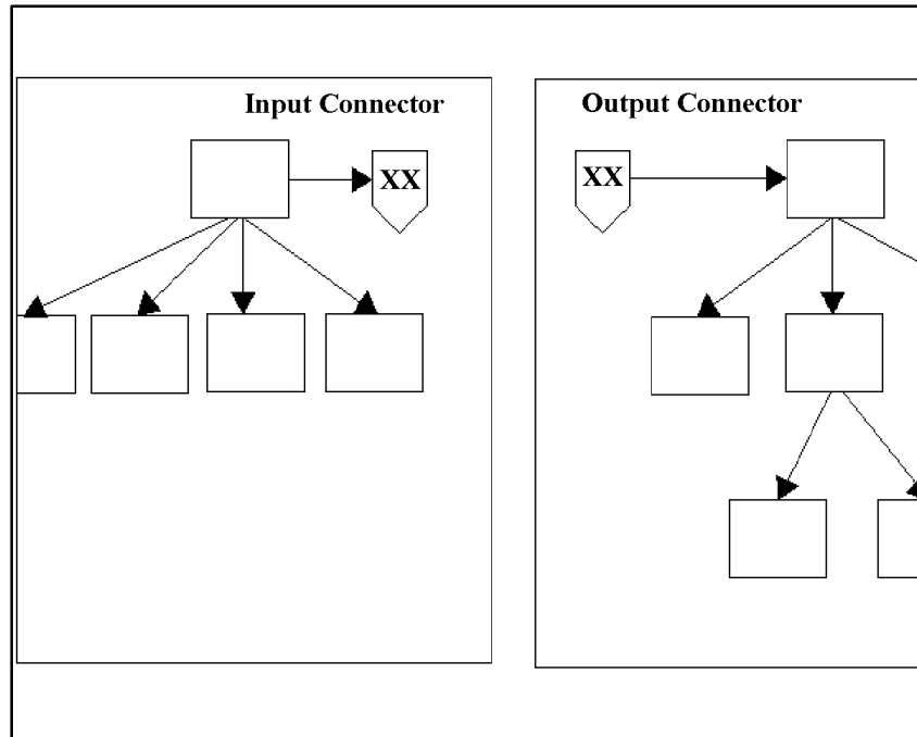
Figure 3-45 Off-Page Connector
