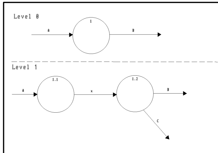
Figure 4-7 Data Flow Errors
