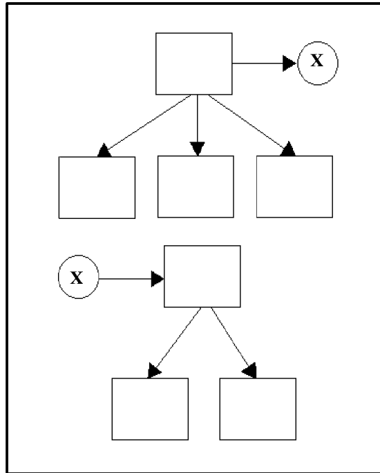
Figure 3-44 On-Page Connectors
