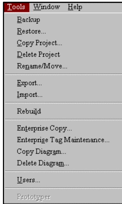
Figure 7-1 Tools Menu
