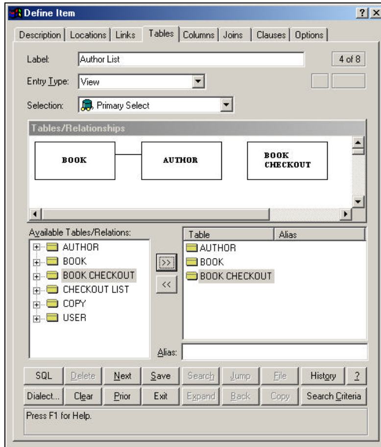
Figure 5-13 Define Dialog Box, View Tables Tab
