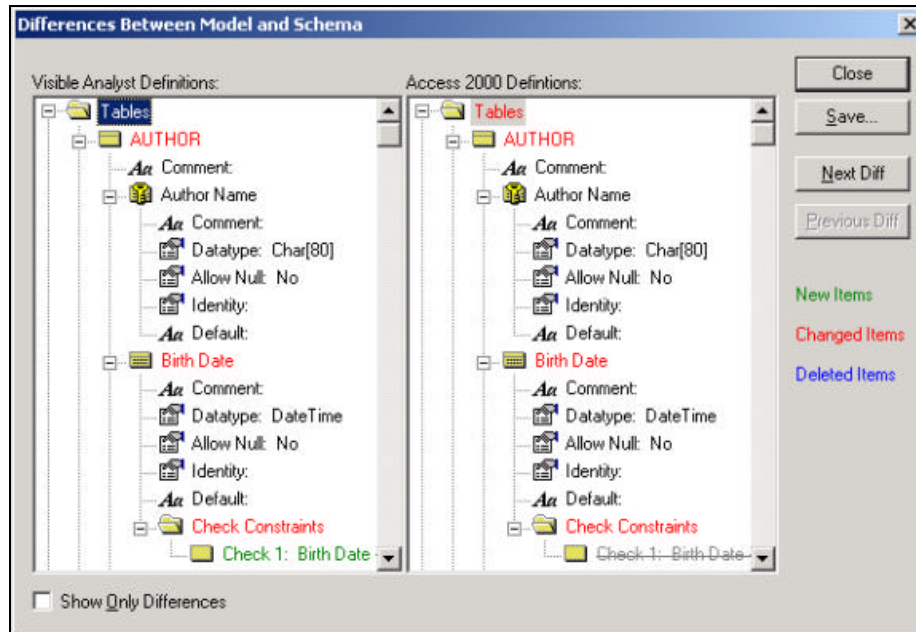
Figure 5-35 Differences Between Model and Schema Dialog Box
