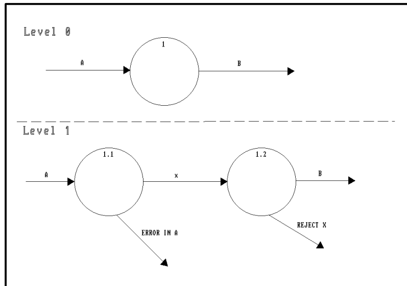
Figure 4-8 Data Flows with Error Labels
