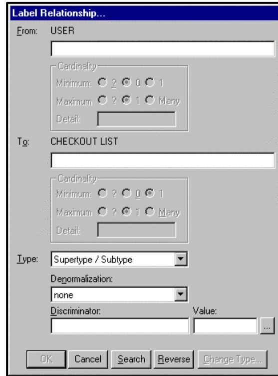
Figure 3-32 Label ERD Relationship Dialog Box
