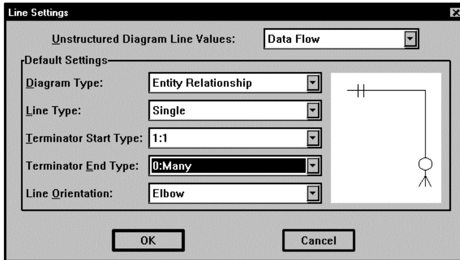
Figure 3-30 Line Settings Dialog Box
