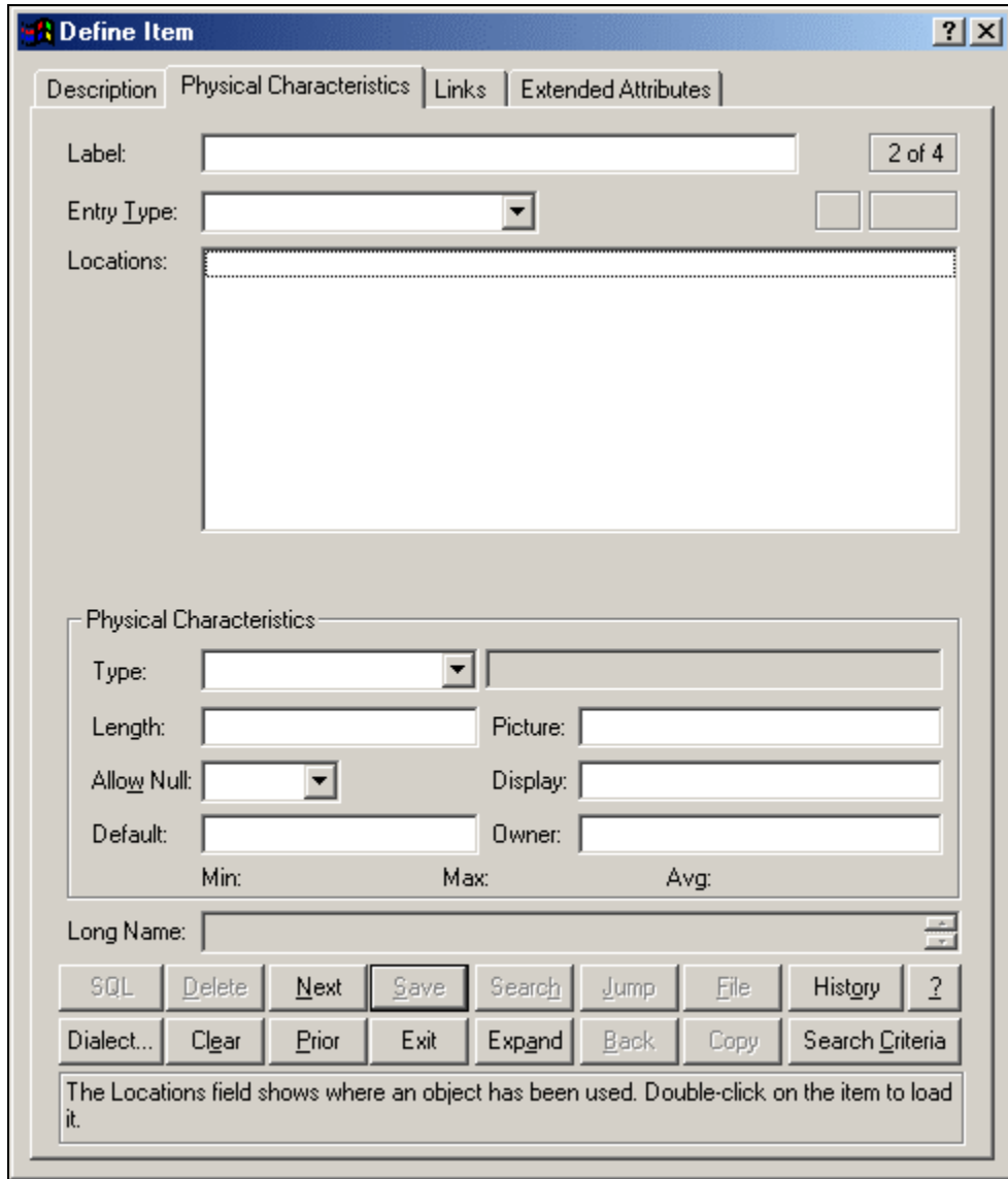
Figure 5-6 Repository Dialog Box, Page 2, Physical Characteristics Tab
