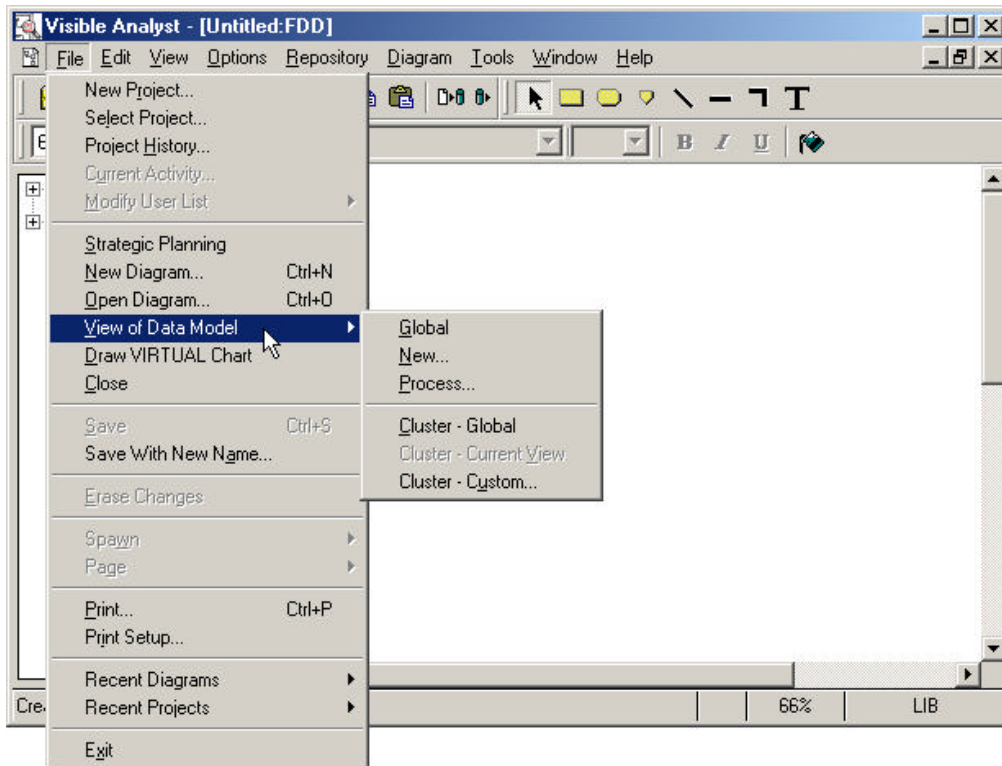
Figure 3-41 The View of Data Model Menu
