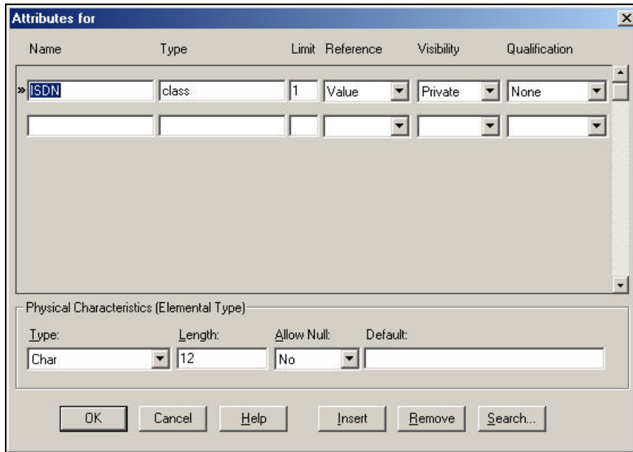
Figure 5-9 Class Attributes
