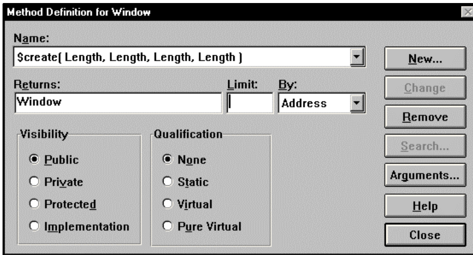
Figure 5-10 Class Methods
